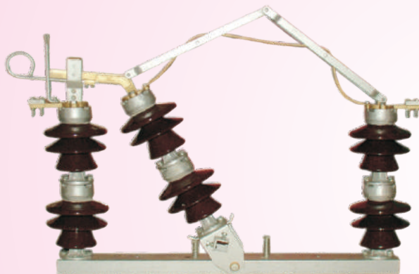
22/33 KV Outdoor triple pole Tilting type, Gang Operated Air Break Switch with Double Stack of Insulator Suitable for horizontal / vertical mounting with complete operating mechanism. Test as per IS-9920 / 1985
