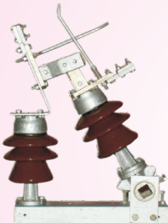
11/22/33 KV Outdoor triple pole Two insulator per pole tilting type, Gang Operated Air Break Switch Suitable for horizontal / vertical mounting with complete operating mechanism. Test as per IS-9920 / 1985
