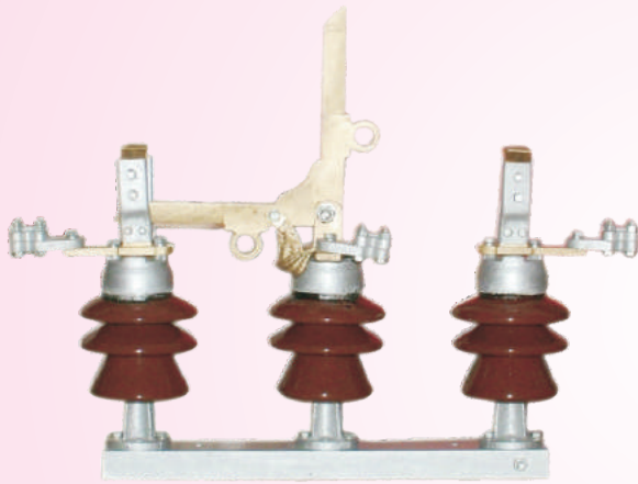
11/22/33 KV Outdoor Three insulator per pole tilting type, Gang Operated Single Phase Switch Suitable for horizontal / vertical mounting. Test as per IS-9920 / 1985
