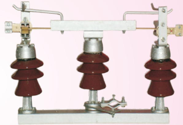
11/22/33 KV Outdoor triple pole Three insulator per pole Rotating type, Gang Operated Air Break Switch Suitable for horizontal mounting with complete operating mechanism. Test as per IS-9920 / 1985
