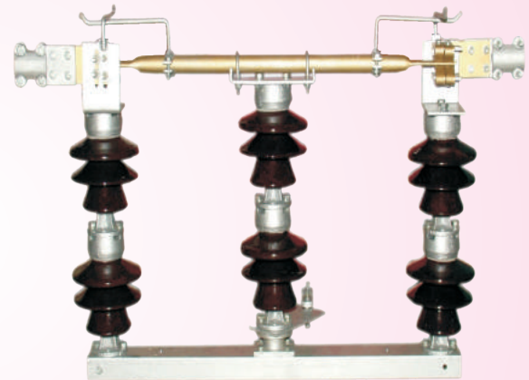
22/33 KV Outdoor triple pole Six insulator per pole Rotating type, Isolator Double Stack of Insulator Suitable for horizontal mounting with complete operating mechanism. Test as per IS-9920 / 1985
